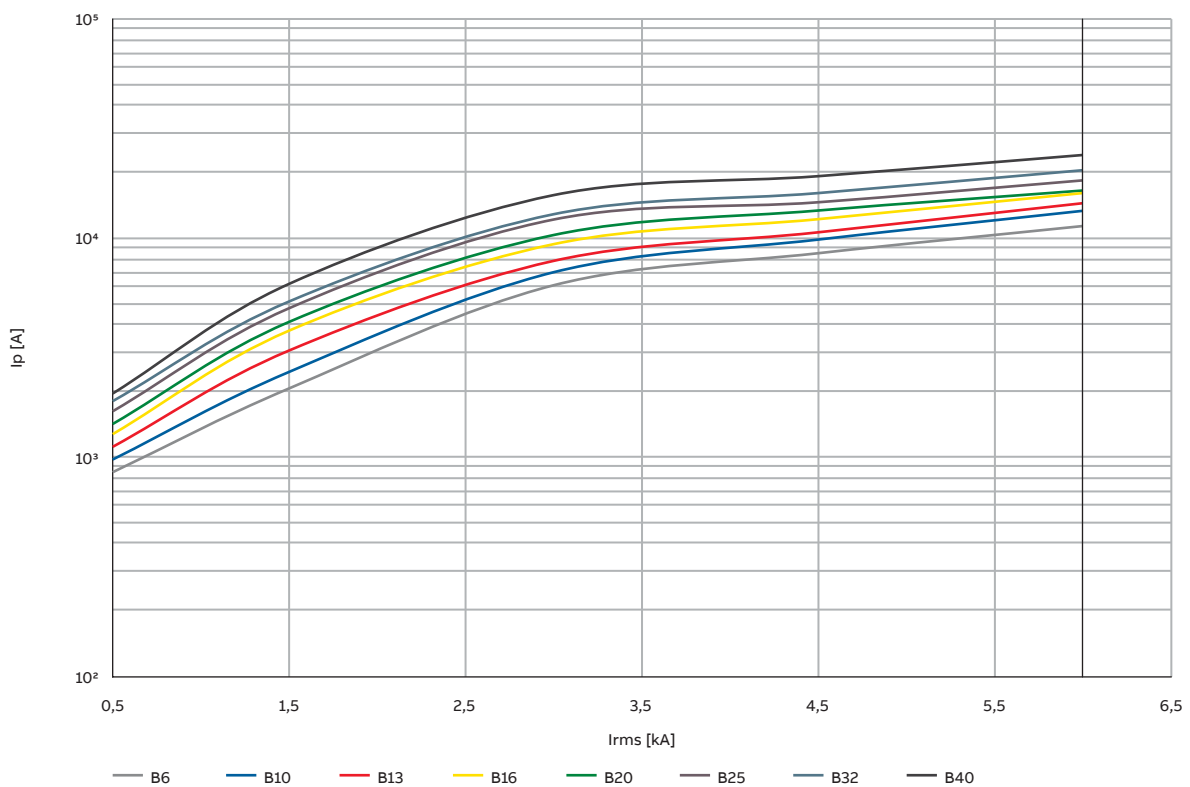
I_{peak} DS201 - Characteristic B
